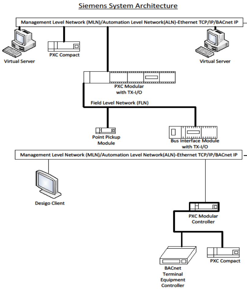
Figure 3: Building Automation System with Siemens Apogee product:
