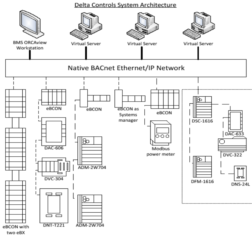
Figure 2: Building Automation System with Delta Controls product:
