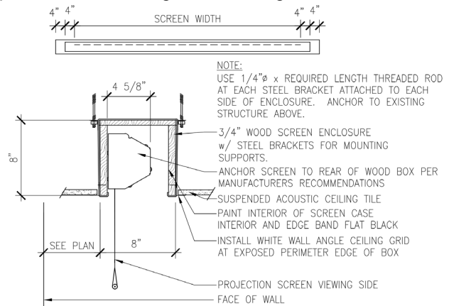
2 RECESSED PROJECTION SCREEN MOUNTING A1.01 SCALE: 1 1/2" = 1'-0"
